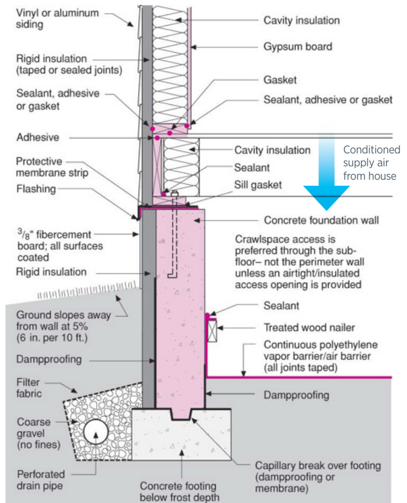
Insulating along the exterior wall is one option for an unvented crawlspace.
